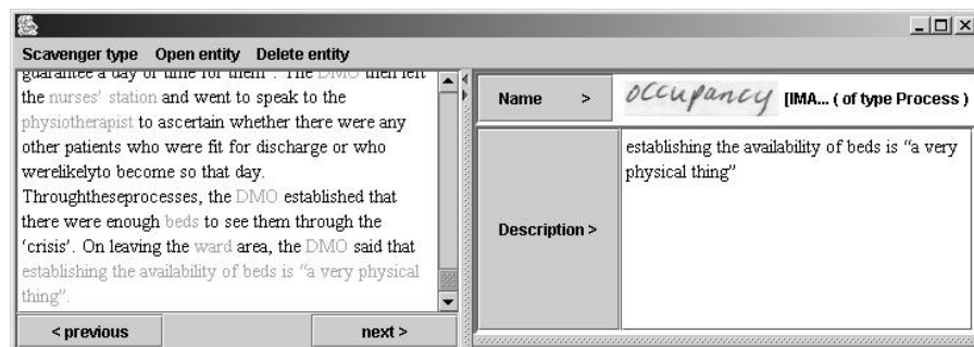
Fig. 3 Entity editor
